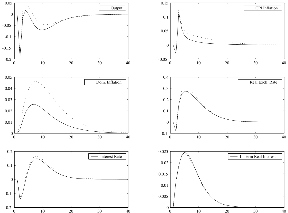
Figure 3: Response of Domestic Variables to a 1% Foreign Inflation Shock (dotted line: Rule with \rho_q = 0 ; continous line: Rule with \rho_q > 0 )
