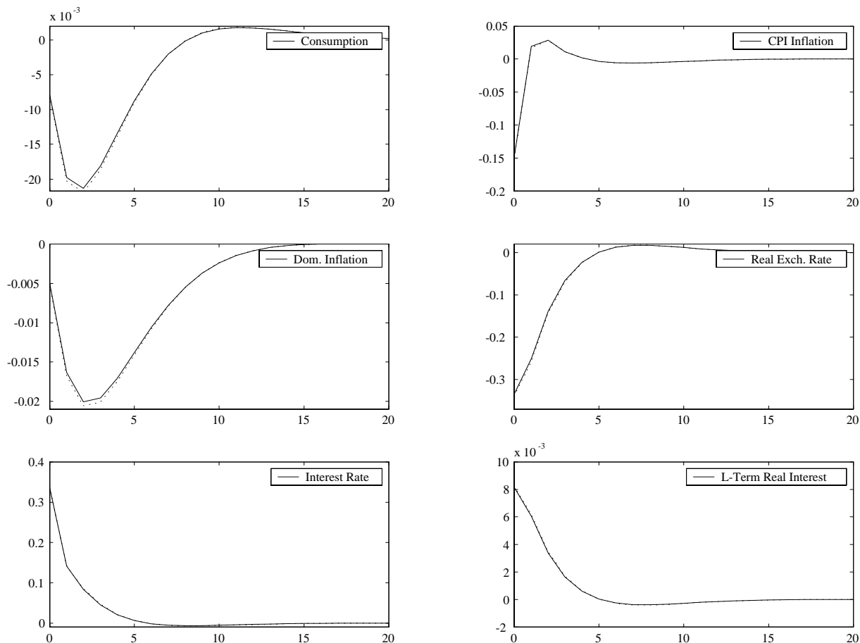
Figure 4: Response of Domestic Variables to a 1% Domestic Interest Rate Shock (dotted line: Rule with \rho_q = 0 ; continous line: Rule with \rho_q > 0 )
